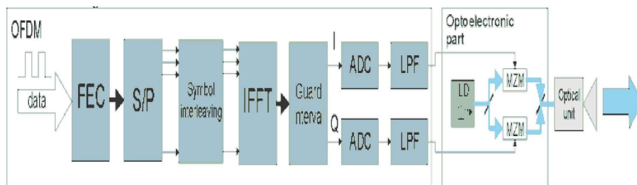
Figure 4. Block diagram of an OFDM FSO system
