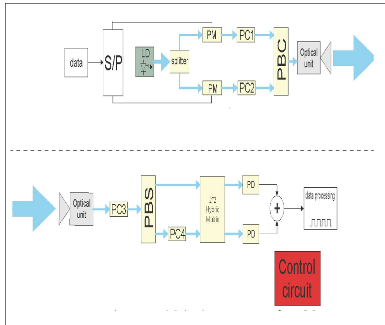
Figure 6. Polarization Multiplexing system for FSO
