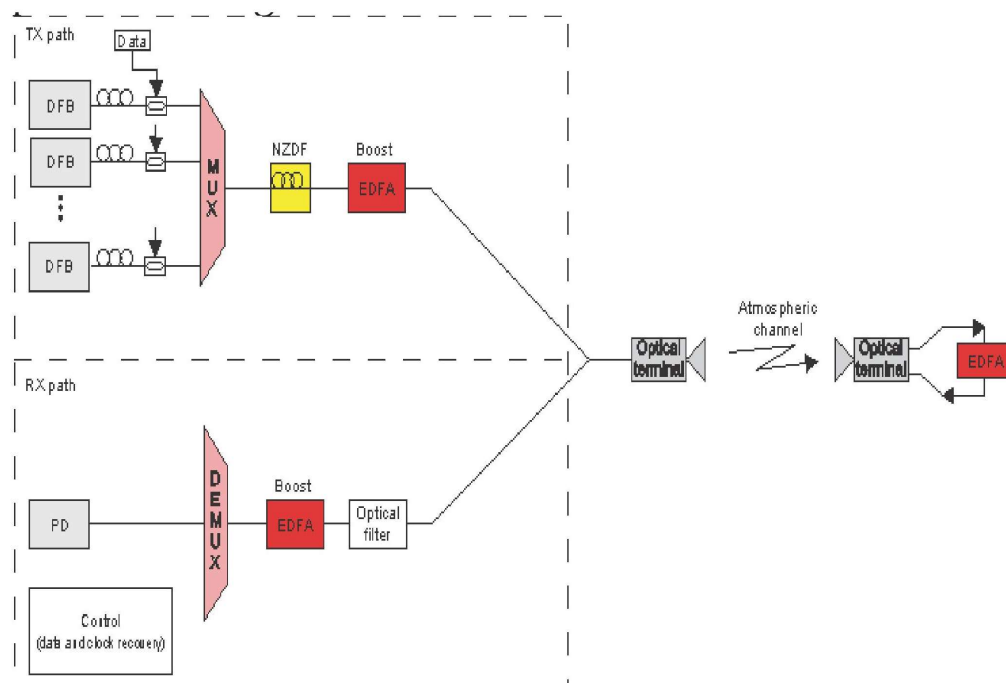
Figure 1. Block diagram of DWDM FSO system
