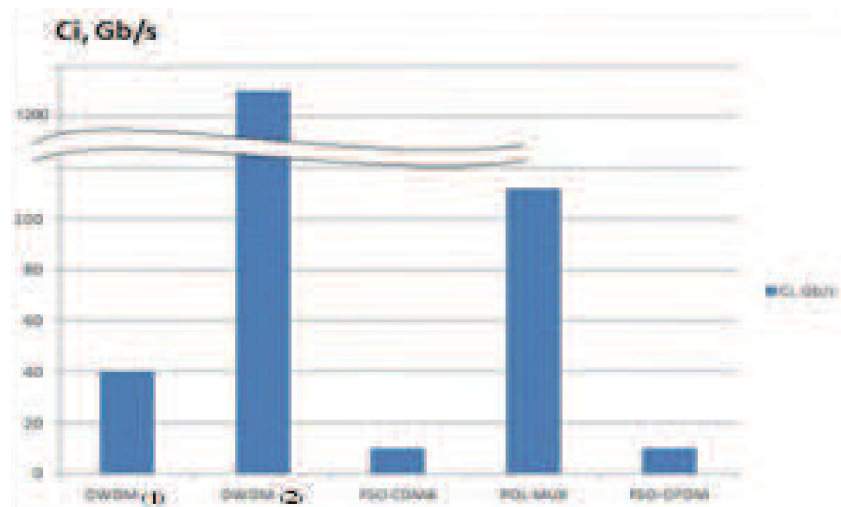
Figure 7. C_I achieved by using different methods for increasing the channel capacity of FSO systems
