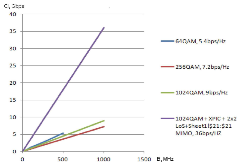
Figure 8. Channel capacity achieved by microwave communication systems
