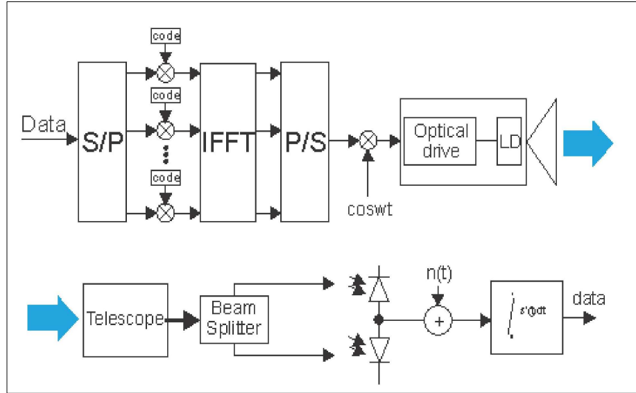
Figure 3. Depicts the code division multiplexing process, that is used in free-space optics
