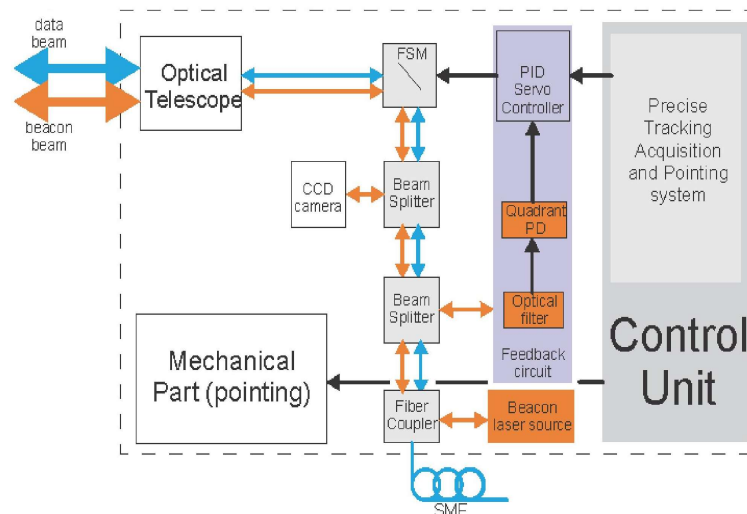
Figure 2. Block diagram of the optical unit
