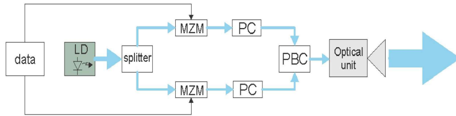
Figure 5. Light polarizing optical terminal for FSO-OFDM systems
