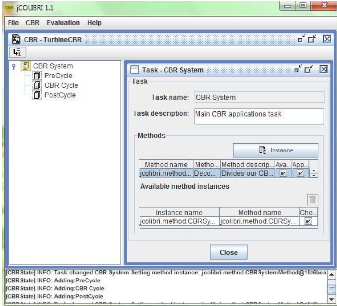
Figure 5(a). Configuration the CBR Application
