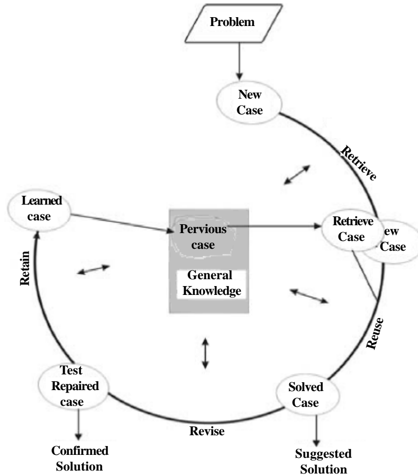
Figure 1. Case based reasoning phases
