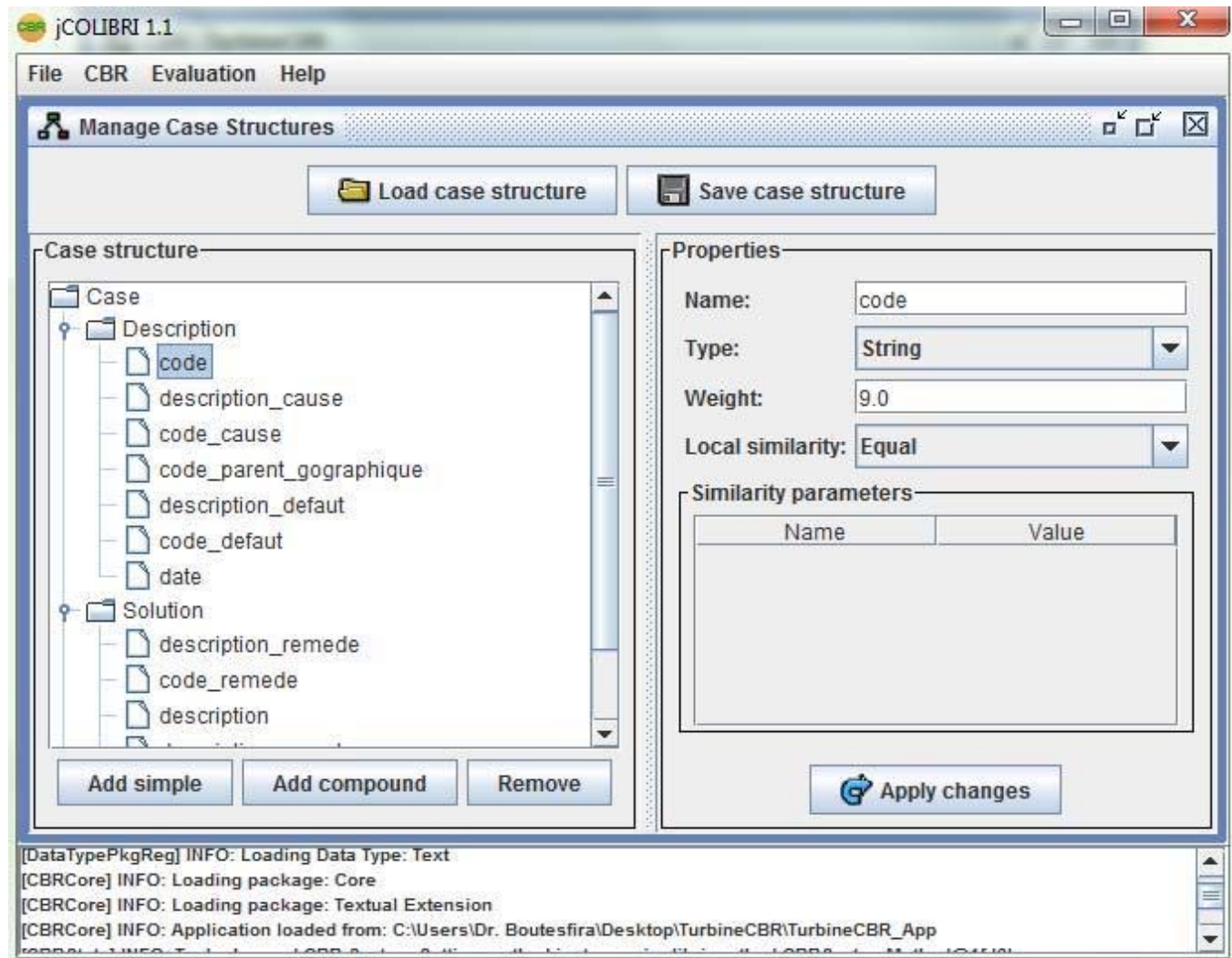
Figure 3. Creation of the case structure
