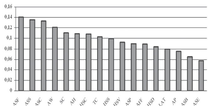
Figure 1. The WALDI graph of the MPEG-7 descriptors. High values indicate high expressiveness.
