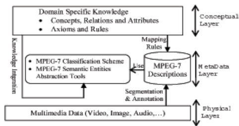
Figure 1. Architecture of the multimedia data representation framework
