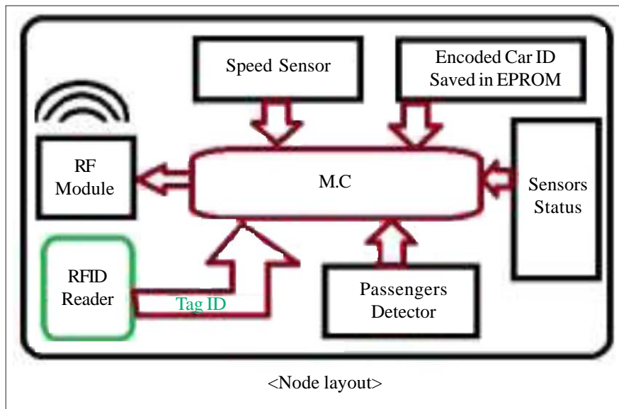
Figure 4. Node layout
