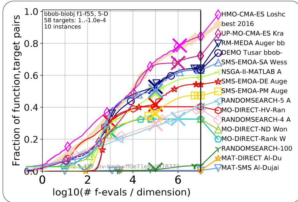
Figure 1. Bootstrapped empirical cumulative distribution of the number of objective function evaluations divided by dimension for 58 targets with target precision in f100; \{10^0, 10^{-0.1}, \dots, 10^{-4.9}, 10^{-5}, 0, -10^{-5}, -10^{-4.8}, \dots, -10^{-4.2}, -10^{-4}\} for 16 algorithms on all 5-D functions of the bbob-biobj test suite
