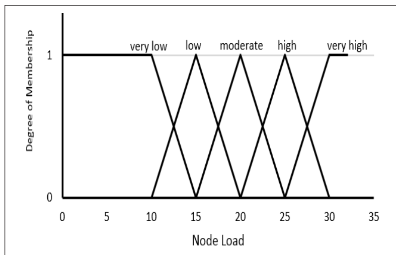
Figure 6. Fuzzy functions for the load of node (output)
