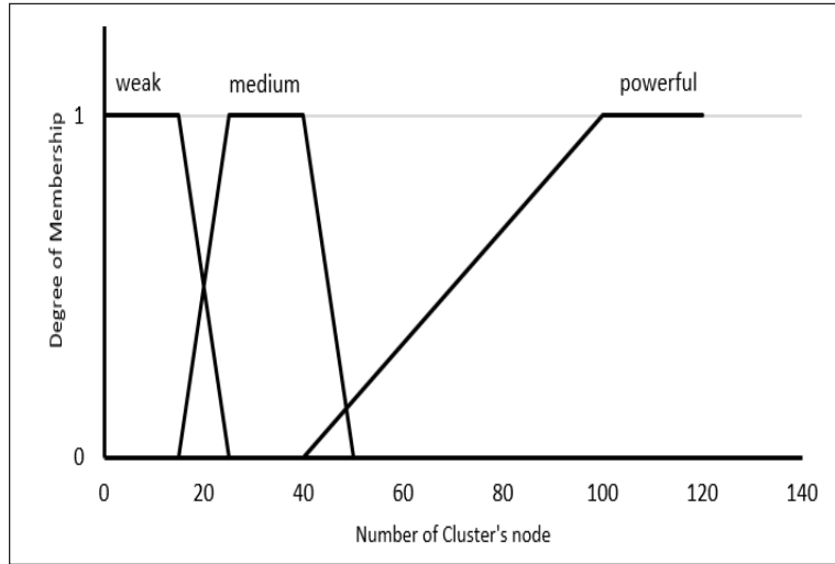
(b) Cluster-power
