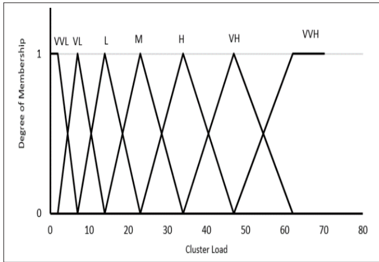
Figure 3. Fuzzy functions for the load of cluster (output)
