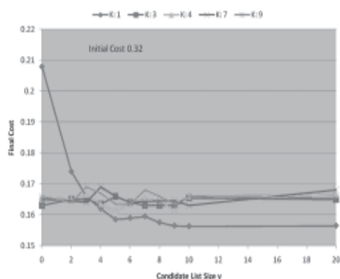
Figure 3. Performance of Tabu Search
