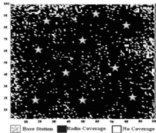
Figure 10. Best Final Solution for the Optimization of Base Station Locations
