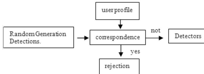
Figure 5. Phase I of the negative selection (generation of detections)
