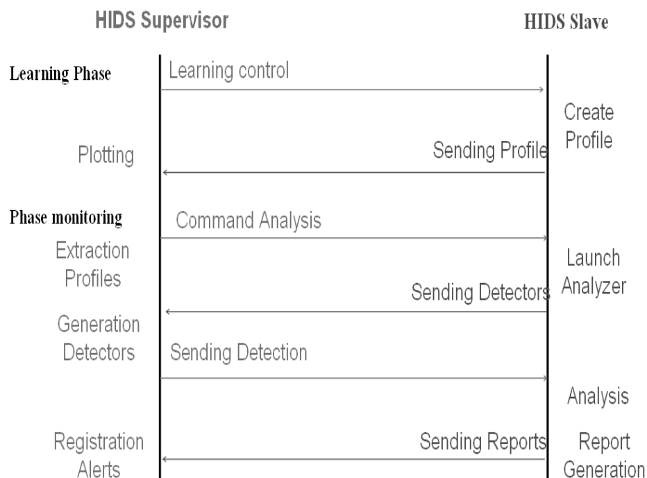
Figure 7. Mode of operation HIDPS
