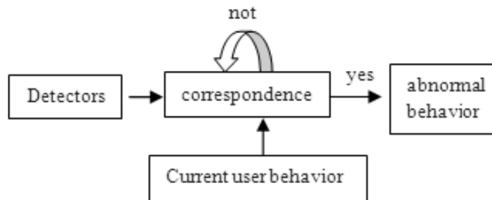
Figure 6. Phase II of negative selection
