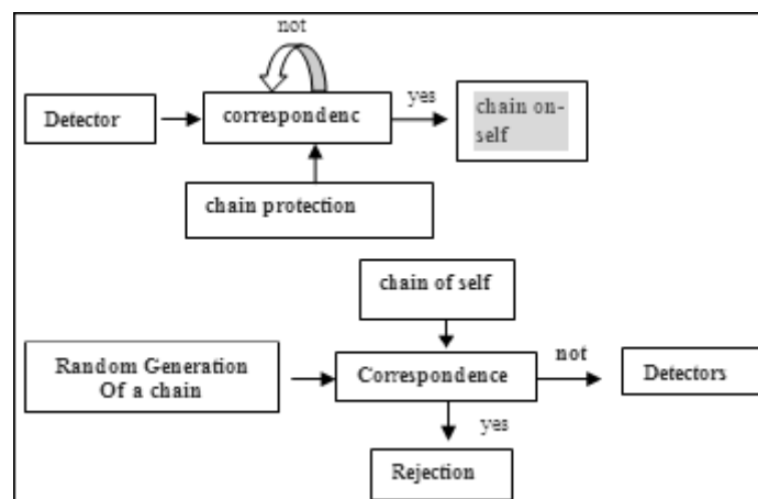
Figure 2. The method of negative selection
