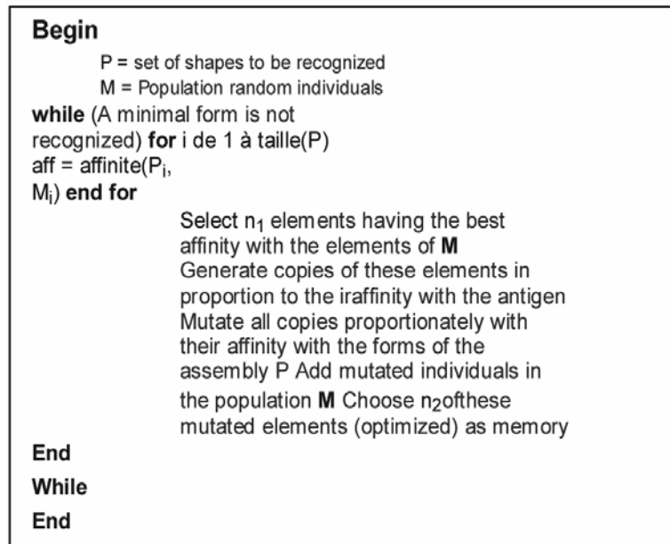
Figure 1. Clonal selection algorithm
