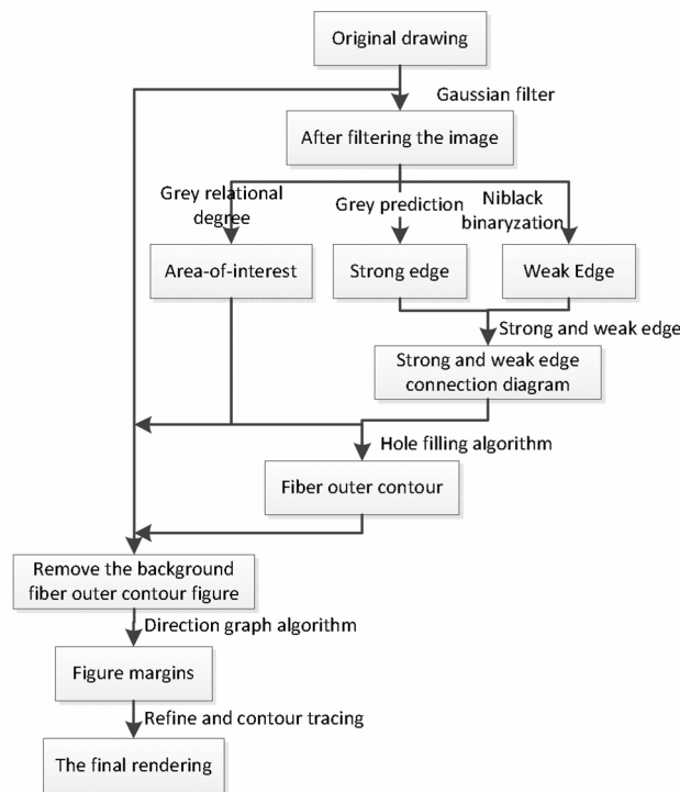
Figure 2. The algorithm process
