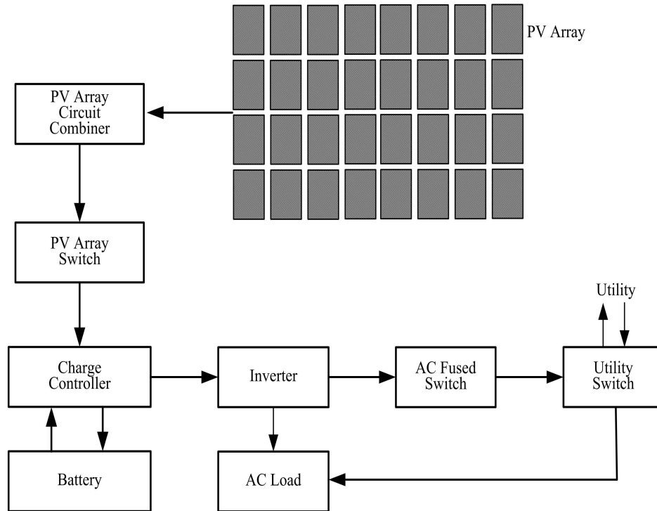
Figure 2. Principle of operation of the designed solar PV system
