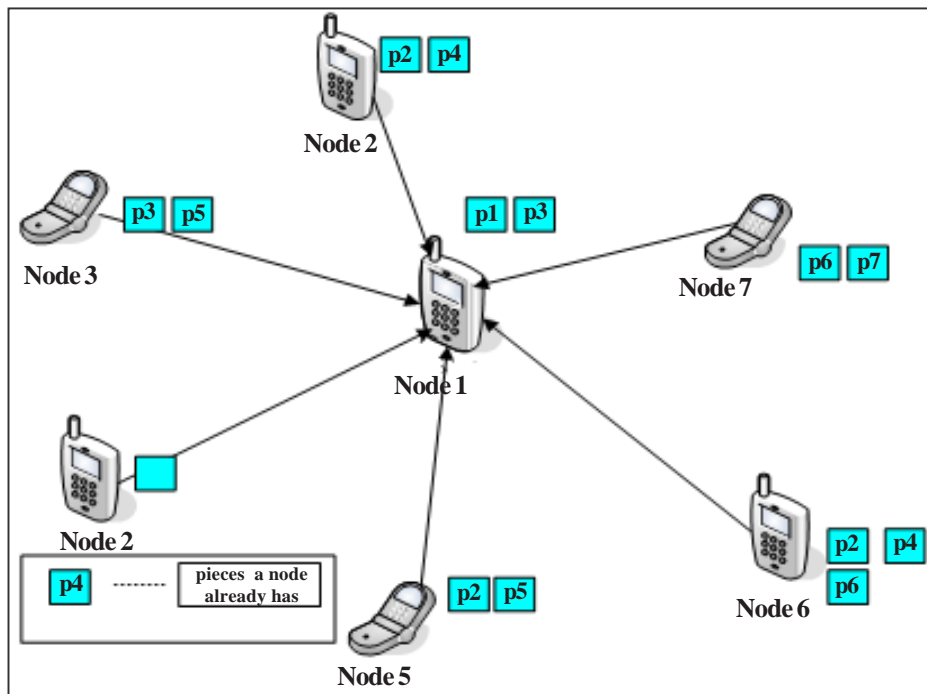
Figure 4. A bad solution of piece downloading
