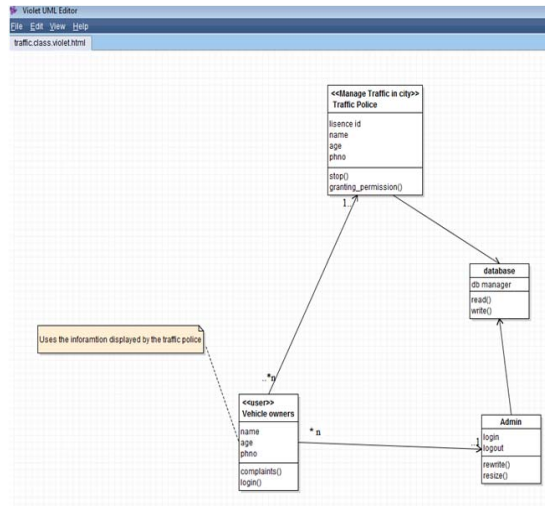
Figure 3. Class Diagram of RTMS
