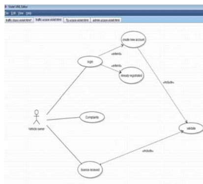
Figure 1. Use case Diagram of Vehicle owner
