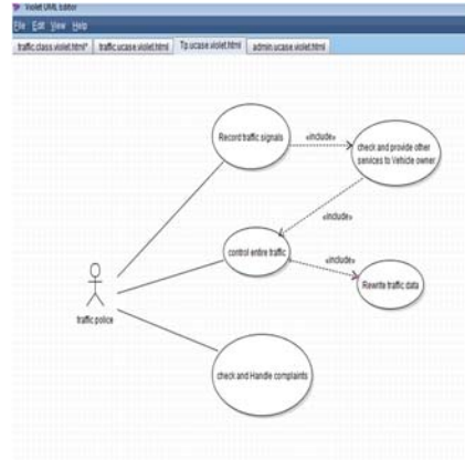
Figure 2. Use case Diagram of Traffic Police
