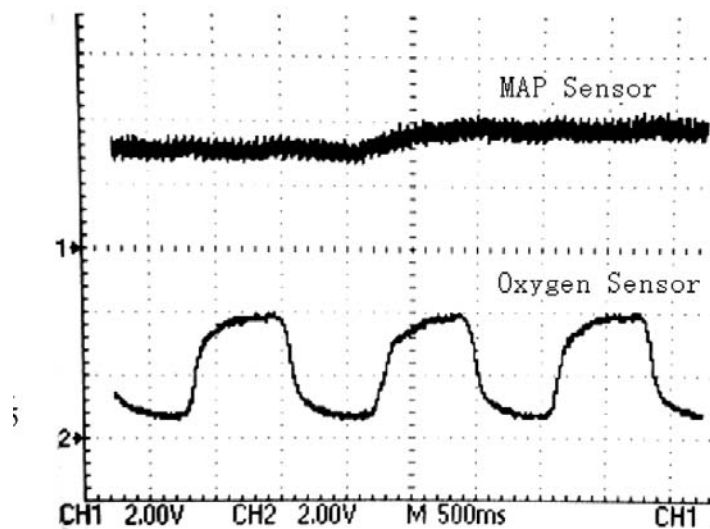
Figure 5. The output of manifold absolute pressure sensor and oxygen sensor (engine speed:2000r/min. intake manifold vacuum:0.032Mpa→0.02Mpa)
