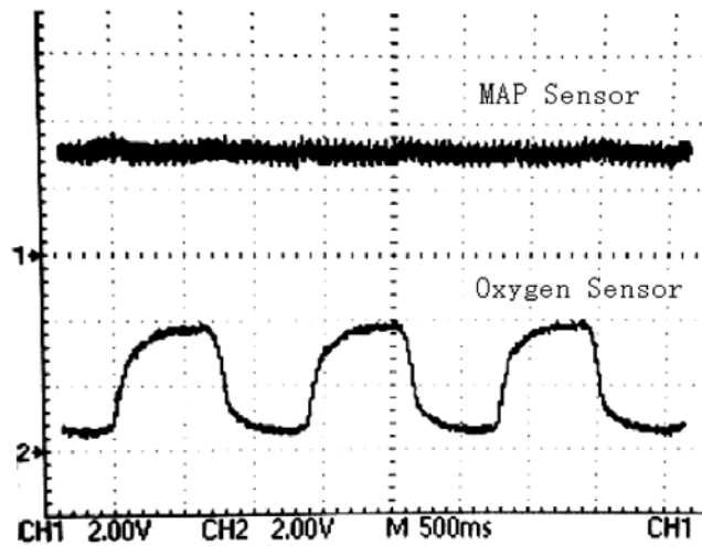
Figure 4. The output of manifold absolute pressure sensor and oxygen sensor (engine speed:2000r/min. intake manifold vacuum:0.032Mpa)
