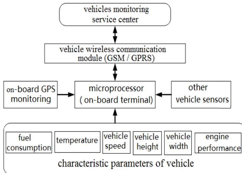
Figure 1. Vehicle safety warning system structure diagram
