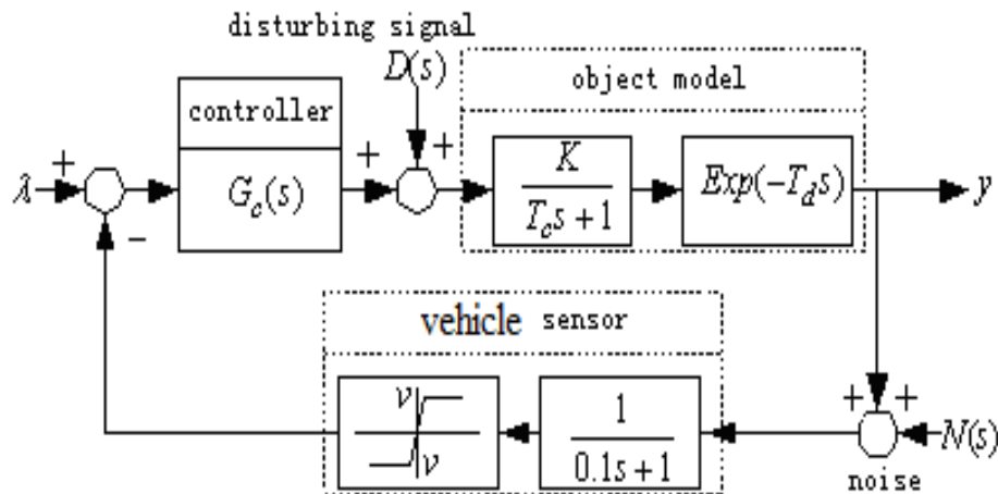
Figure 3. Closed loop control system
