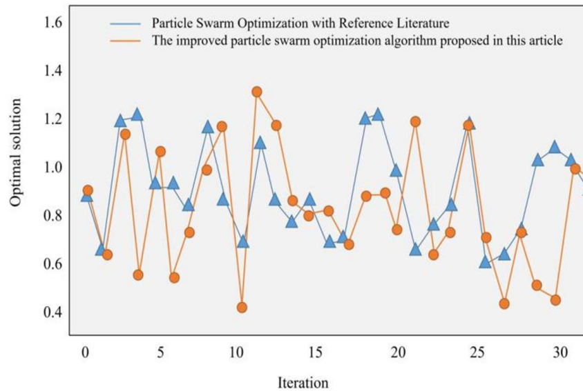
Figure 3. Optimal Solution of the Objective Function
