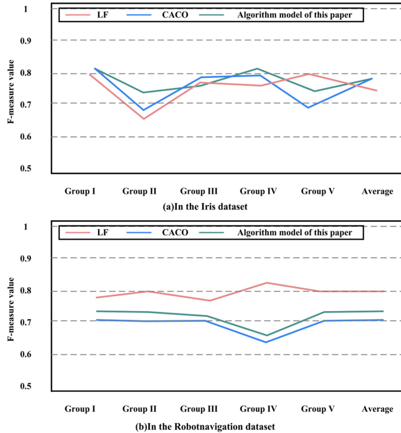
Figure 1. Comparison of F-measure values of three algorithms in two different datasets
