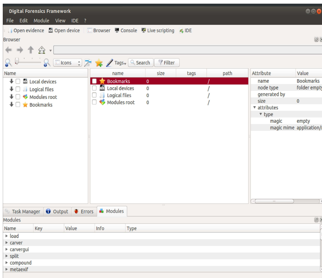
Figure 1. DFF analysis of evidence
