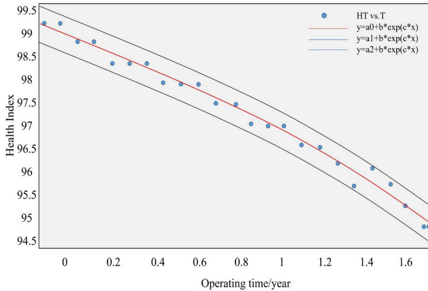
Figure 1. Changes in Health Index (HI) of Control Center Components over Time
