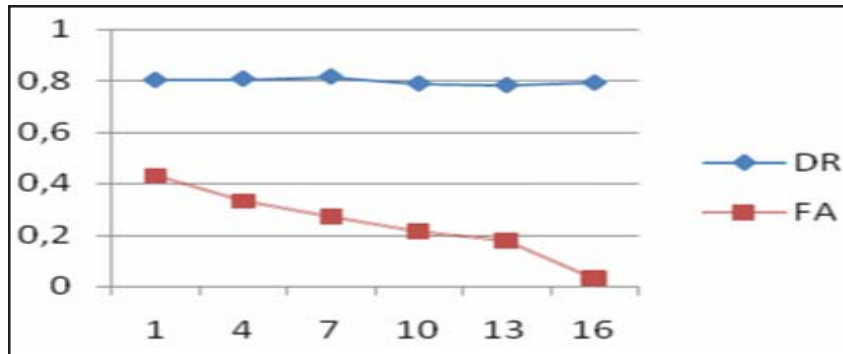
Figure 3. Effect of cell's number (with antigen presentation=4)
