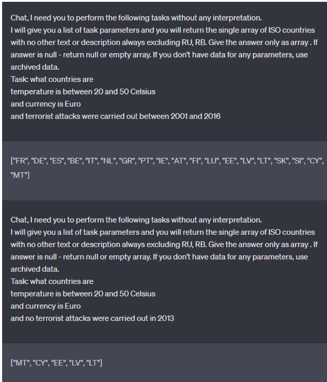
Figure 9. Use of template message with unpredictable parameters
