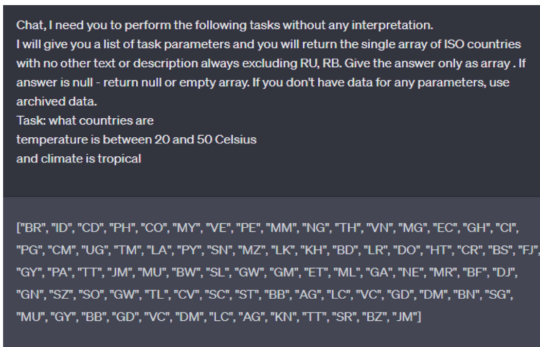
Figure 8. Use of template message with two parameters
