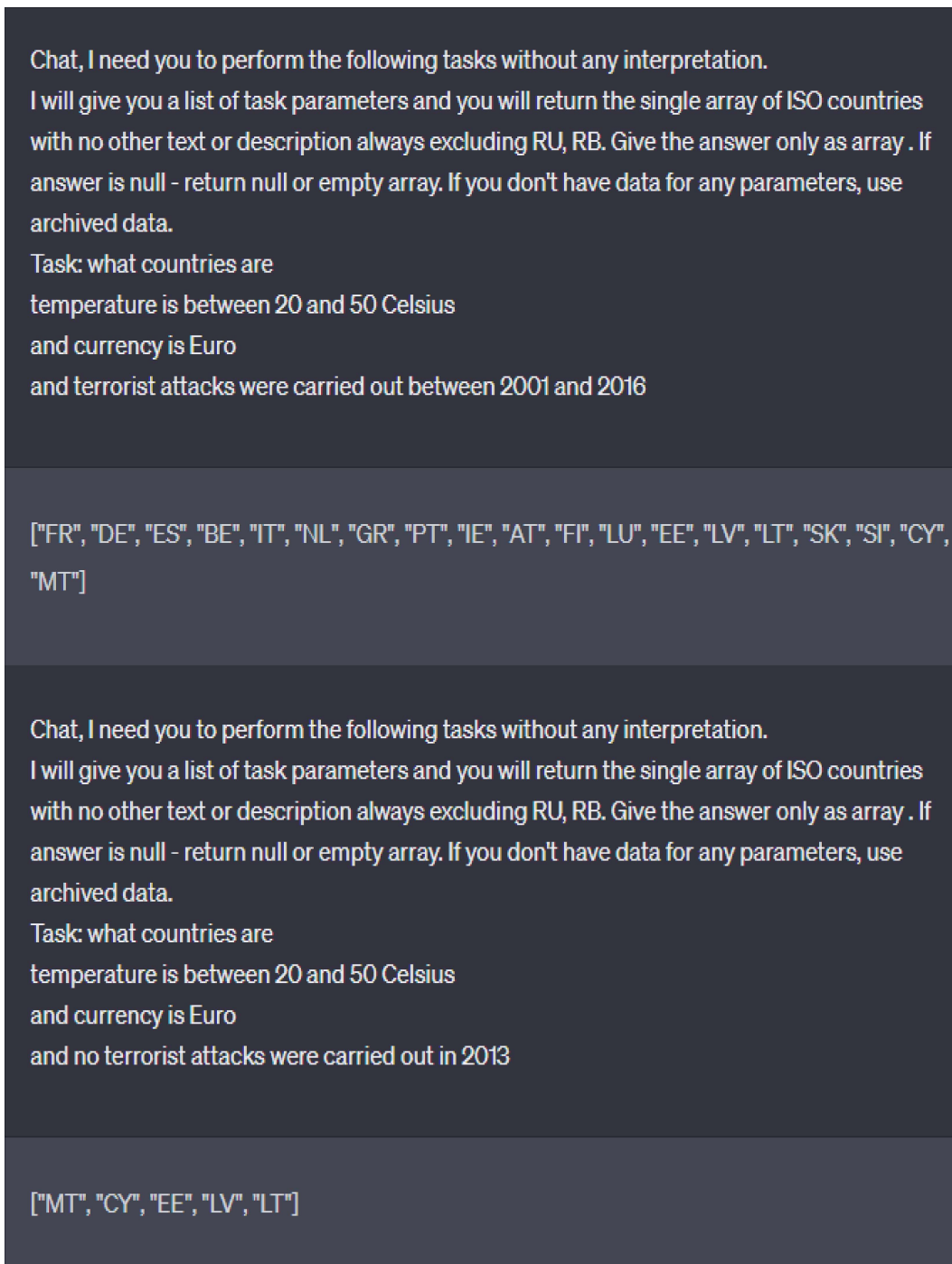
Figure 10. Use of template message with unpredictable parameters
