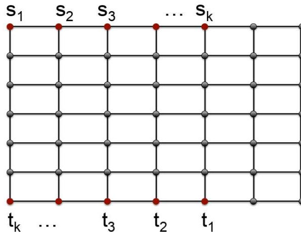
Figure 2. Integrality gap example
