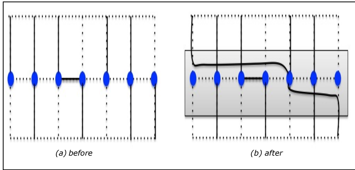
Figure 5. Altering the drawing around S_i
