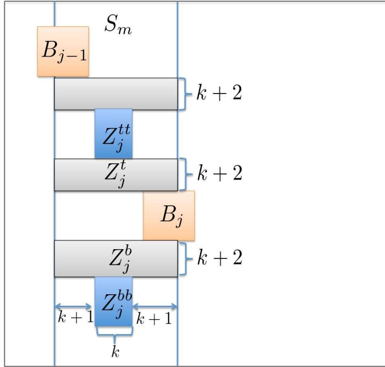
Figure 4 Graphs Z_j^b , Z_j^t , Z_j^{bb} and Z_j^{tt}
