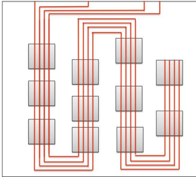
Figure 3. Traversing the boxes
