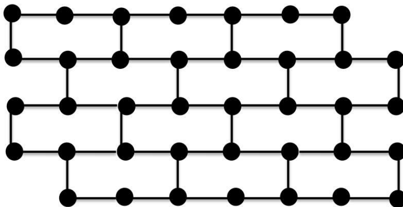
Figure 1. A wall graph
