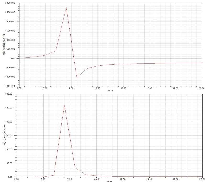
Figure 4. Parasite resonance, depending on the number of wire turns at fixed frequency 75MHz: imaginary (above) and real (bottom) components of the antenna input impedance
