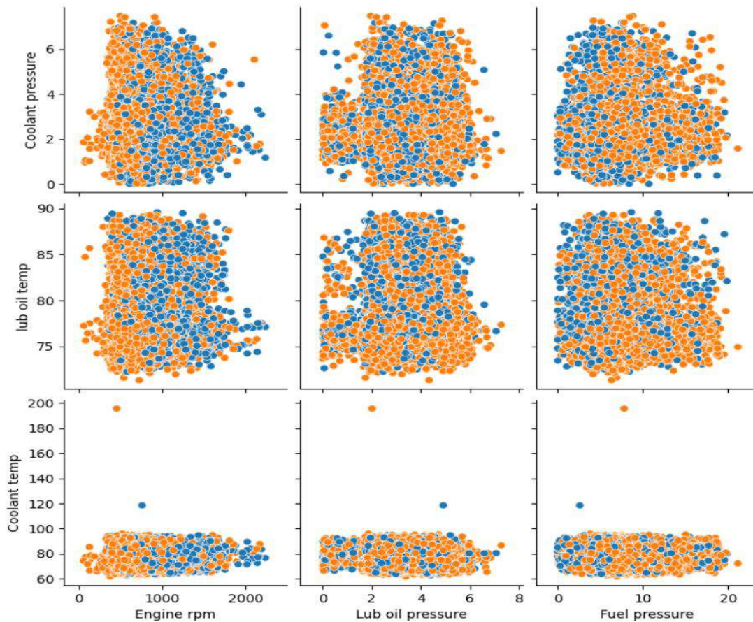
Figure 1. Visual representation of the Automotive Vehicles Engine Health Dataset
