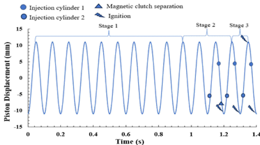
Figure 3. FPE model control method
