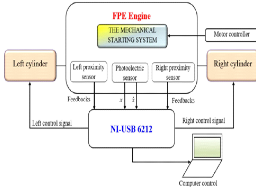
Figure 4. FPE model control structure
