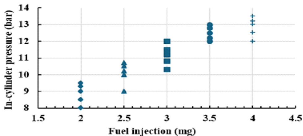
Figure 8. Fuel injection with in-cylinder pressure of the first ignition process
