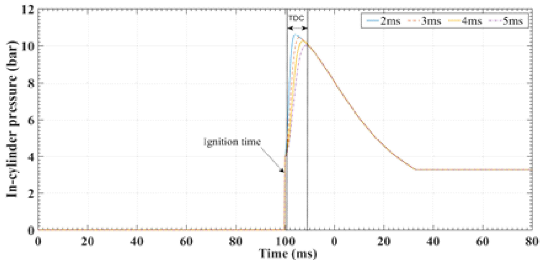
Figure 7. In-cylinder pressure with burn duration time 2 ms -5 ms
