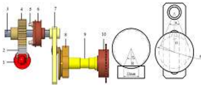
Figure 2. Mechanical starting and Coulissee mechanism
