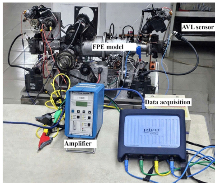
Figure 5. Experimental model of FPE
