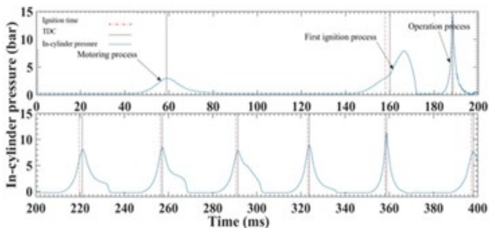
Figure 10. In-cylinder pressure during all processes
